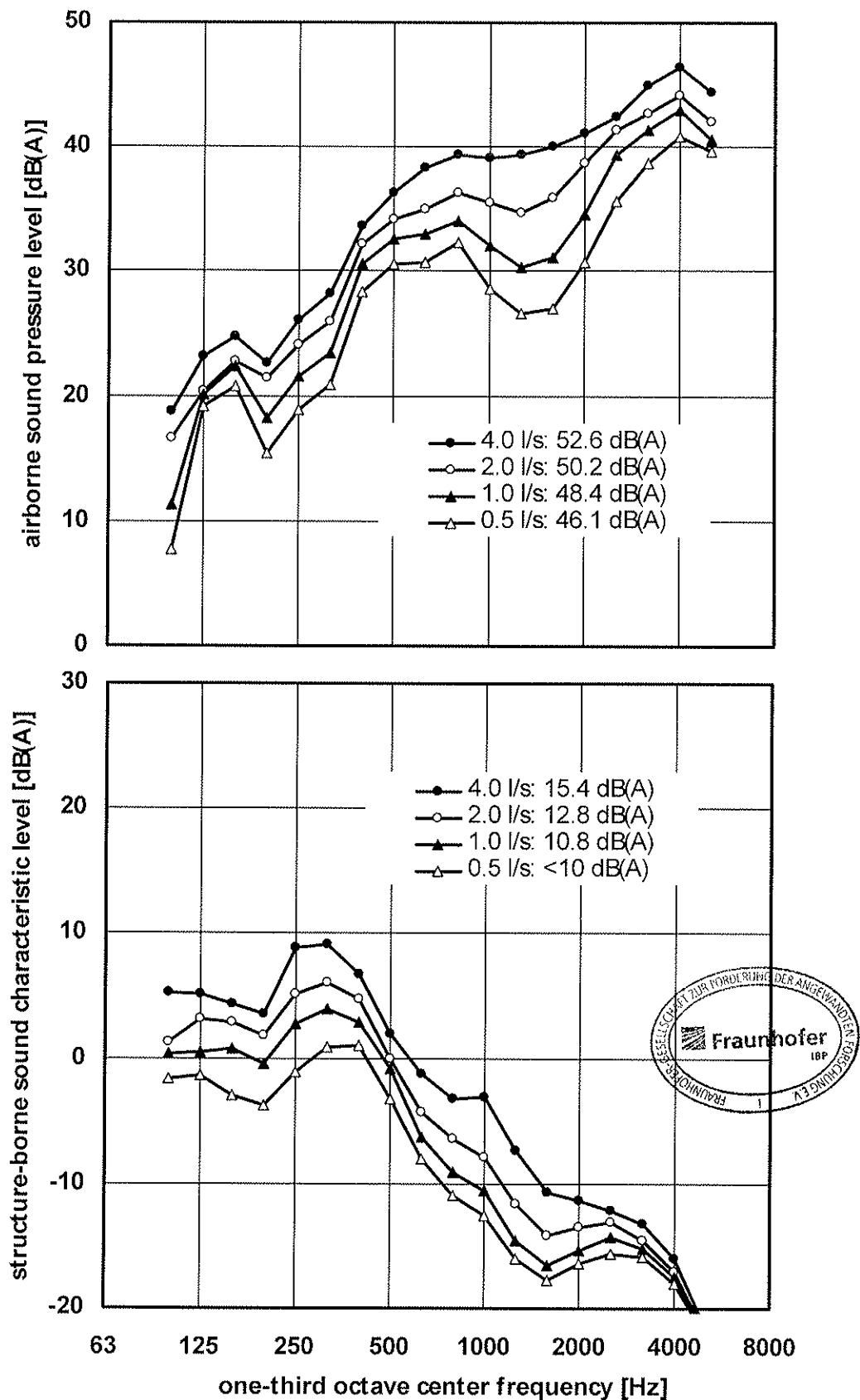
Figure 2 Wastewater pipe system "Ultra Silent+ 110 x 4.8" mounted according to figure 4, using pipe clamps "Müpro yellow, with spacer 5 mm". Airborne sound pressure level (above) and structure-borne sound characteristic level (below) measured at various flow rates according to DIN EN 14366.
