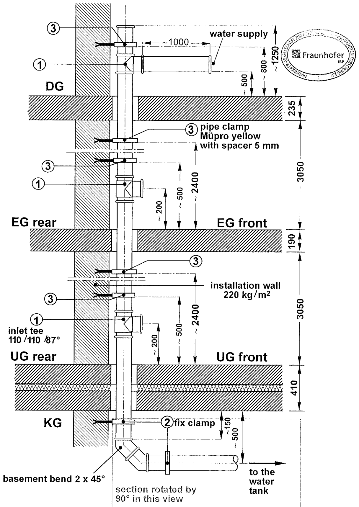
Figure 4 Installation plan of the pipe system "Ultra Silent+ 110 x 4.8" (manufacturer: HULIOT (A.C.S) LTD.), mounted with pipe clamps "Müpro yellow, with spacer 5 mm". Drawing not to scale, dimensions in mm.
