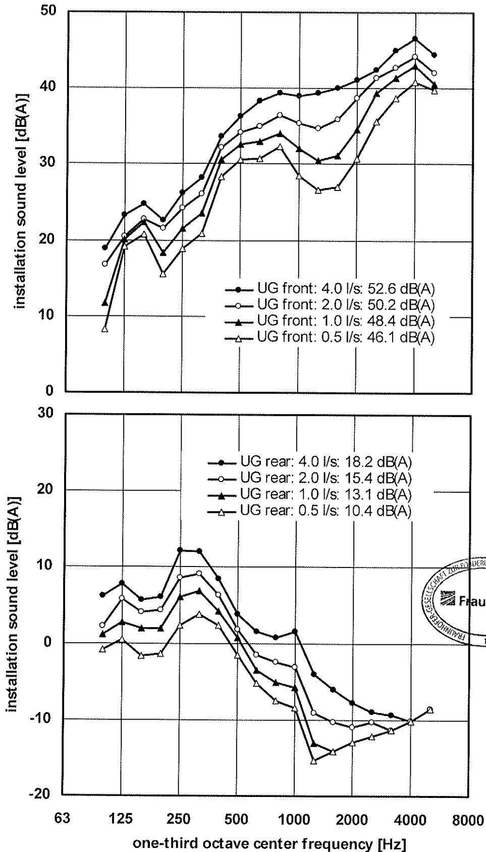
Figure 1 Wastewater pipe system "Ultra Silent+ 110 x 4.8" mounted according to figure 4, using pipe clamps "Müpro yellow, with spacer 5 mm". The installation sound level L_{in} was measured at various flow rates in the test rooms UG front (above) and UG rear (below).
